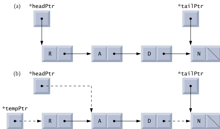
Fig. 12.16 | dequeue operation.
