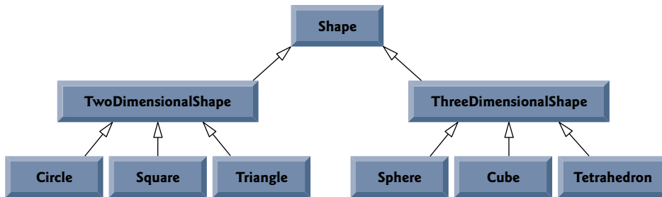
Fig. 19.3 | Inheritance hierarchy for Shapes.
